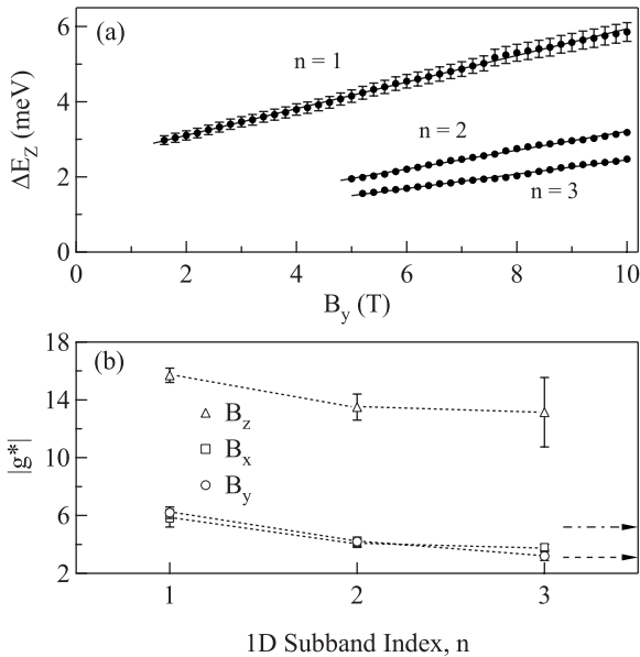
FIG. 2. (a) Zeeman splitting \Delta E_Z plotted vs magnetic field B_y for the lowest three subbands. Solid lines show linear fits to the data. (b) Effective Landé g factors |g^*| measured in the QPC for the three magnetic field orientations B_x , B_y , and B_z . Dashed lines are guides to the eye. The upper and lower arrows on the right-hand side indicate the bare 2D g factors from Ref. 4 for B perpendicular and parallel to the quantum well respectively.
